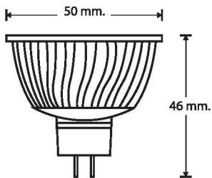
Product Dimension
